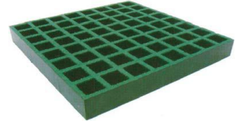
Standard 38 x 38mm Mesh Grating with Grit
